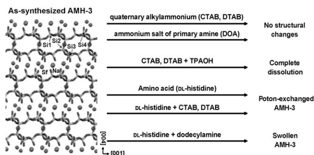
Figure 1. AMH-3 structure projection along the b axis showing silicon atoms (Si1, Si2, Si3, and Si4, light sticks), oxygen atoms (dark sticks), sodium cations (Na, single balls), and strontium cations (Sr, double balls). Details on the structure can be found in reference [5]. The arrows indicate attempted ion-exchange and swelling procedures. Only the last procedure, combination of ion exchange in the presence of DL-histidine and swelling using dodecylamine, resulted in swollen AMH-3. CTAB = cetyltrimethylammonium bromide, DTAB = dodecyltrimethylammonium bromide, DOA = dodecylamine, TPAOH = tetrapropylammonium hydroxide.
