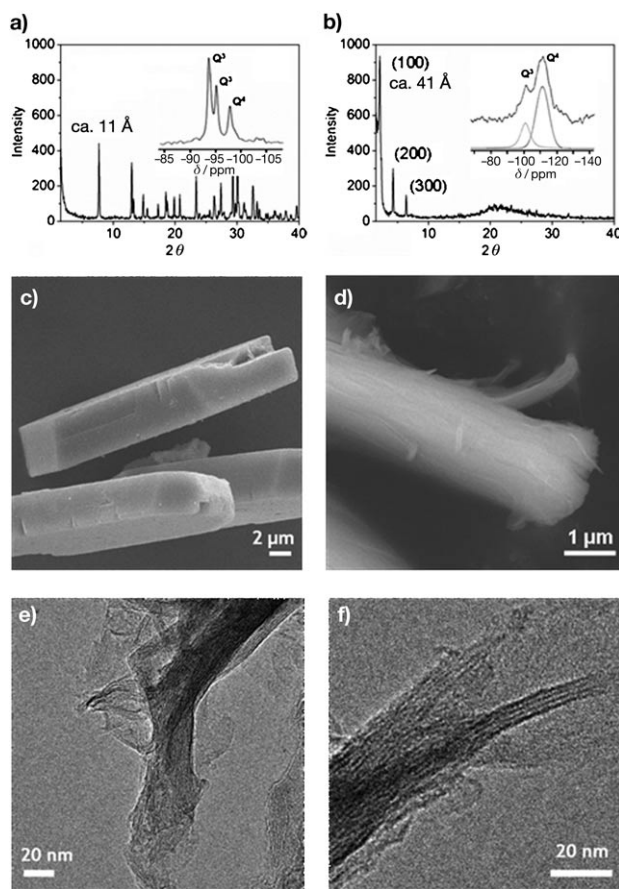
Figure 2. a, b) X-ray diffraction patterns and ^{29}\text{Si} solid-state MAS NMR spectra (inset) of original crystalline (a) and swollen (b) AMH-3. c, d) SEM images of original (c) and swollen (d) AMH-3. e, f) TEM images of swollen AMH-3.
