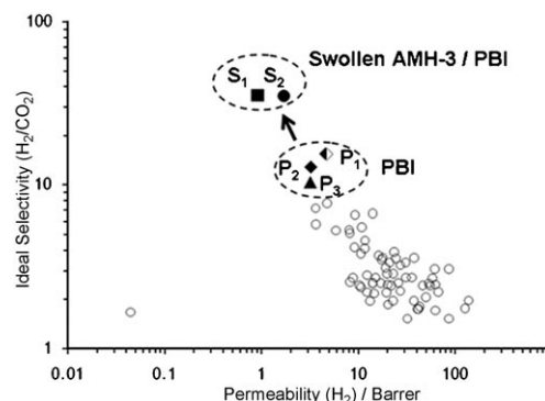
Figure 4. Hydrogen/carbon dioxide ideal selectivity versus hydrogen permeability. Pure PBI from reference [40] ( P_1 ), pure PBI from this work ( P_2 ), PBI with dodecylamine ( P_3 ), and 3 wt % ( S_1 ) and 2 wt % ( S_2 ) swollen AMH-3/PBI nanocomposites. The open symbols denote other glassy polymers from reference [35].
